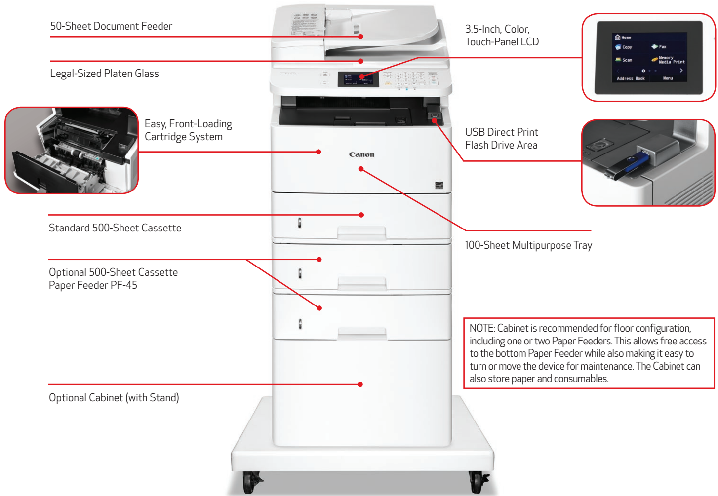
MF515dw shown with two optional Paper Feeders and optional Cabinet Type-M1
