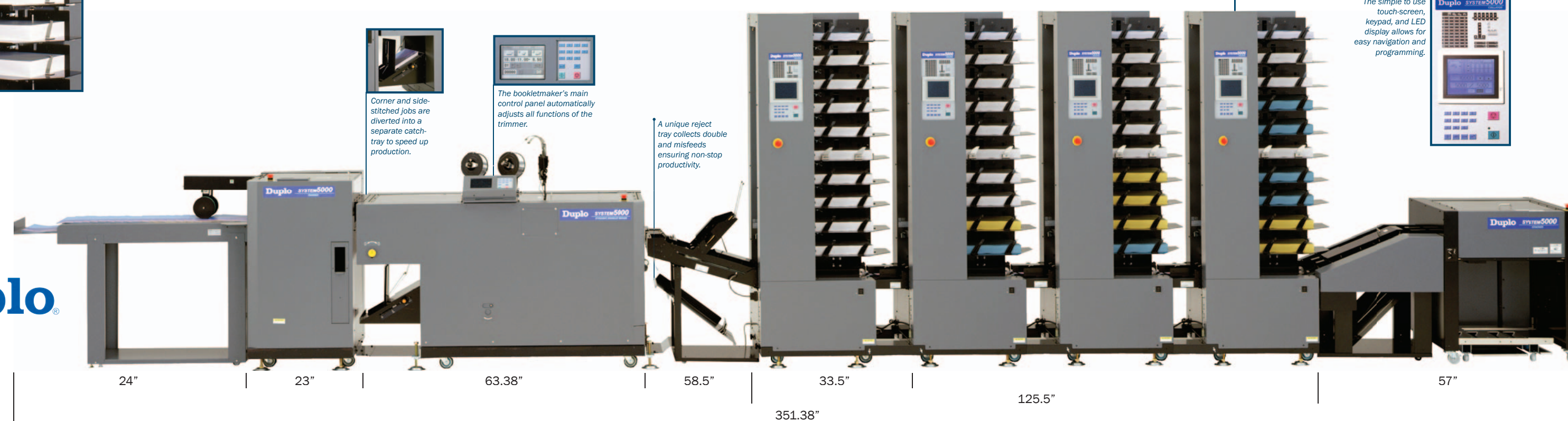
The 2.5" bin capacity conveniently loads 11 lb. to 12-pt. cover stock of paper sizes ranging from 4.72" x 5.52" to 14" x 20".
