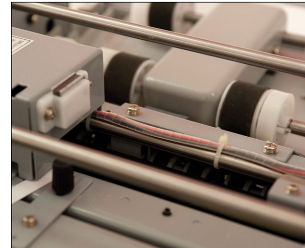
Special feed rollers and separator ensure no double feeds or marking even with matt coated papers
